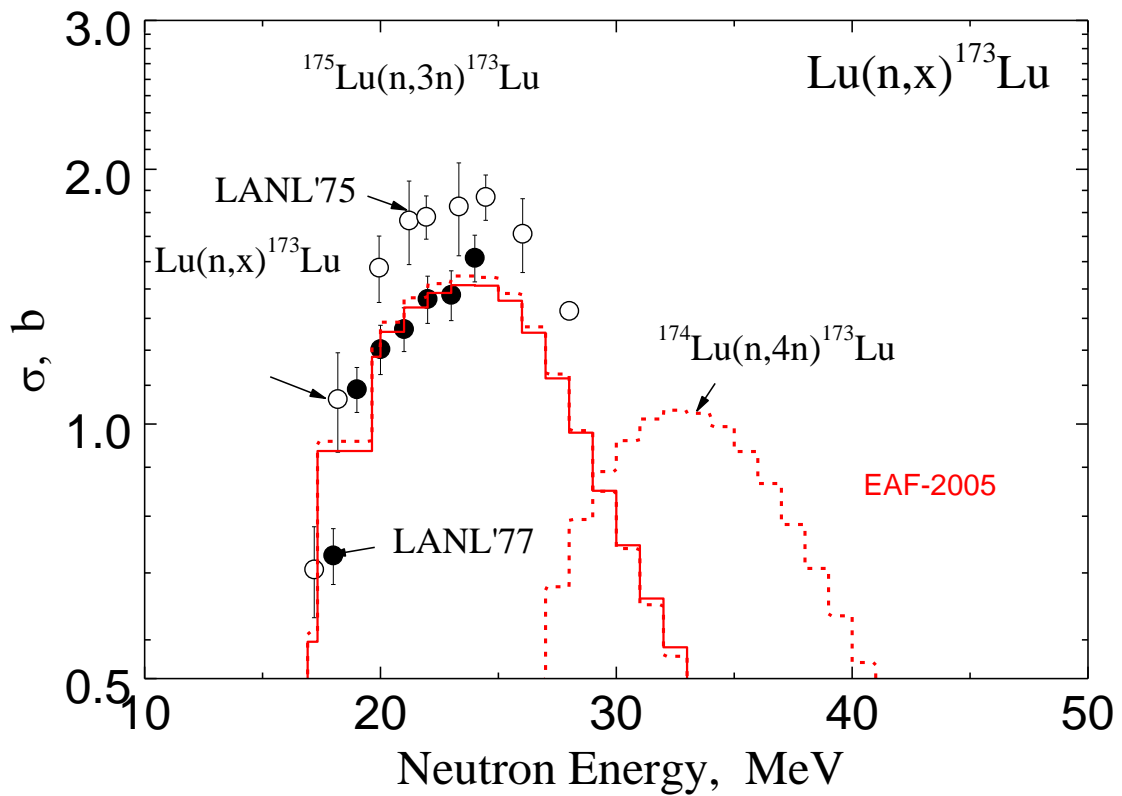
Fig. 2. The ^{175}\text{Lu}(n,3n)^{173}\text{Lu} cross sections
