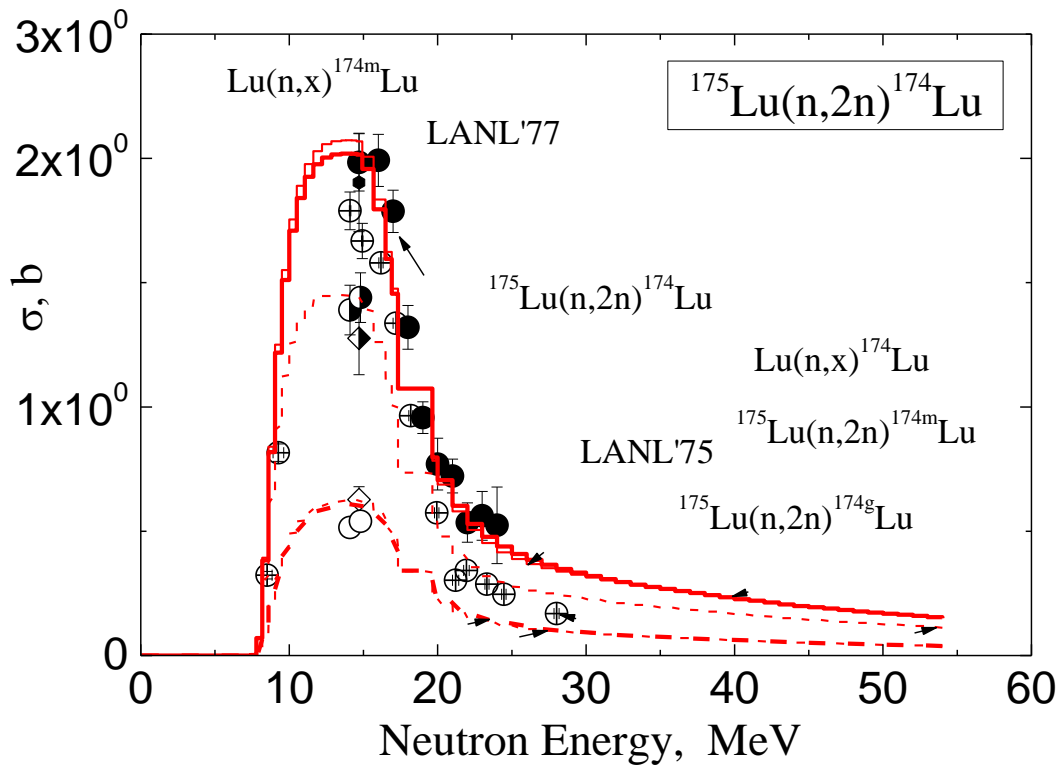
Fig. 1. The ^{175}\text{Lu}(n,2n)^{174}\text{Lu} cross sections
