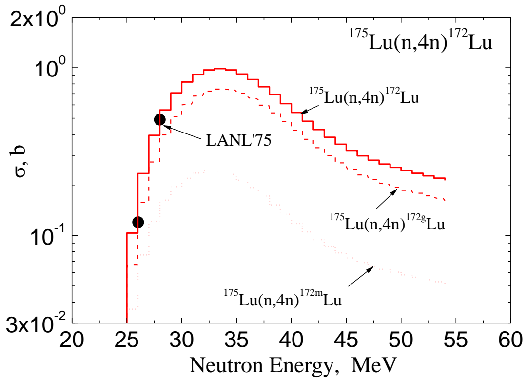
Fig. 3. The ^{175}\text{Lu}(n,4n)^{172}\text{Lu} cross sections.
