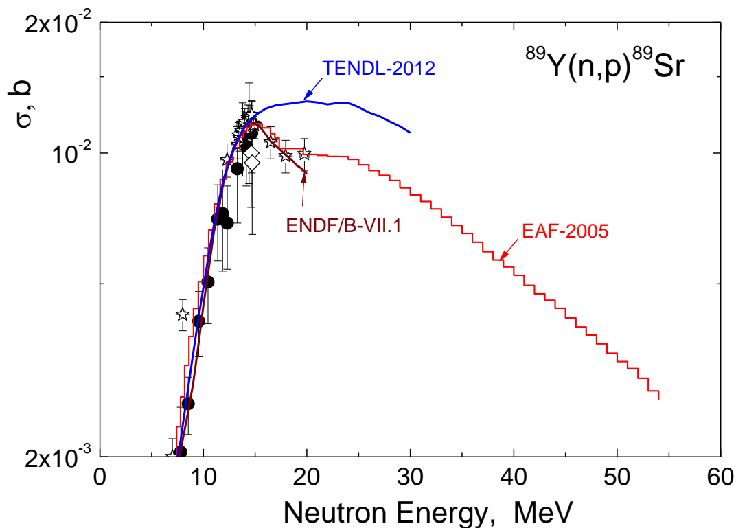
Fig. 4. Experimental and Evaluated data for the ^{89}\text{Y}(n,p)^{89}\text{Sr} cross section.
