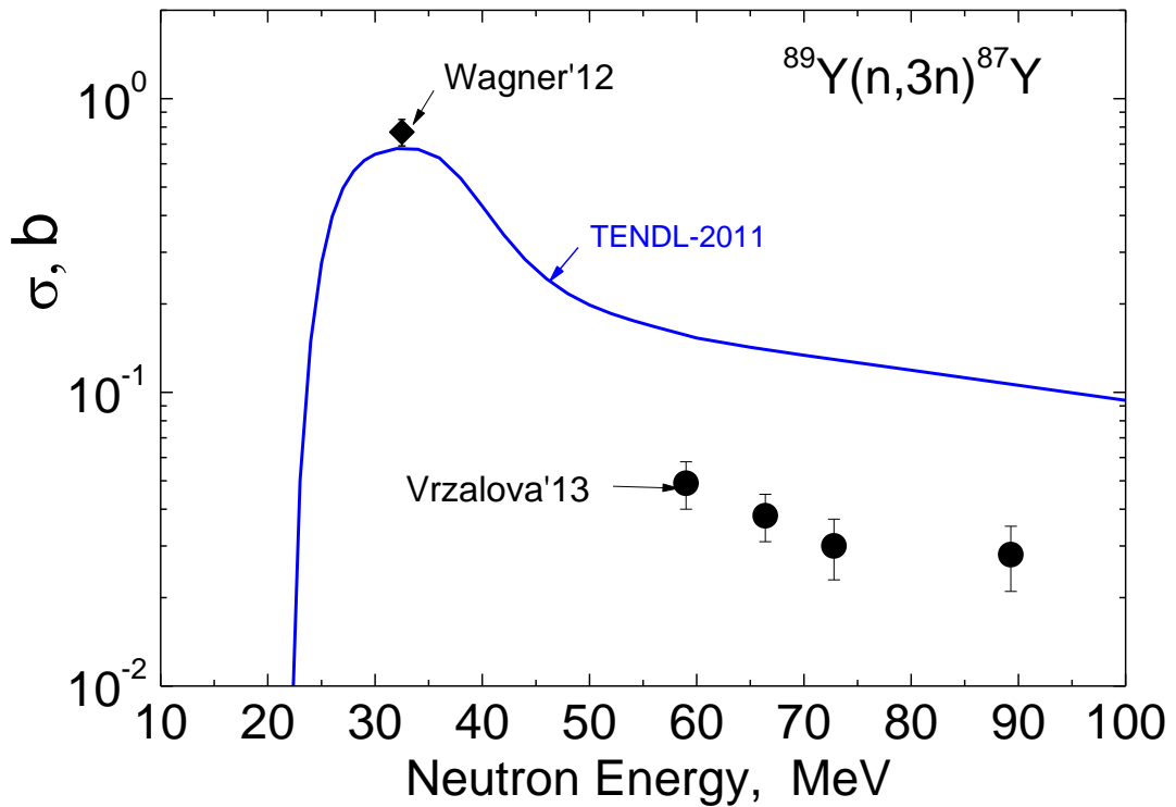
Fig. 2. Experimental and Evaluated data for the ^{89}\text{Y}(n,3n)^{87}\text{Y} cross section.
