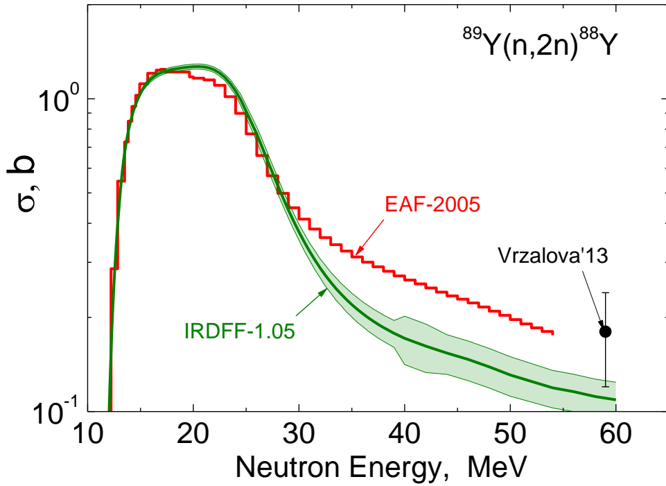
Fig. 1. Experimental (only new measurements, since 2012) and Evaluated data for the ^{89}\text{Y}(n,2n)^{88}\text{Y} cross section.
