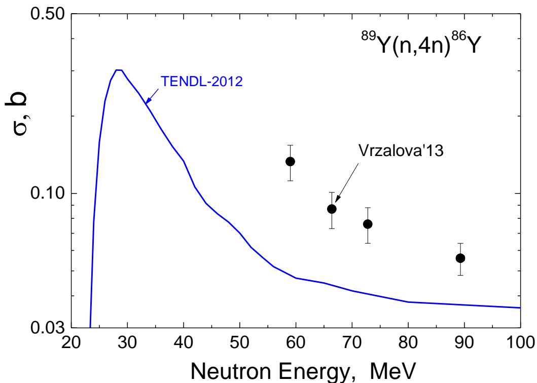
Fig. 3. Experimental and Evaluated data for the ^{89}\text{Y}(n,4n)^{86}\text{Y} cross section.
