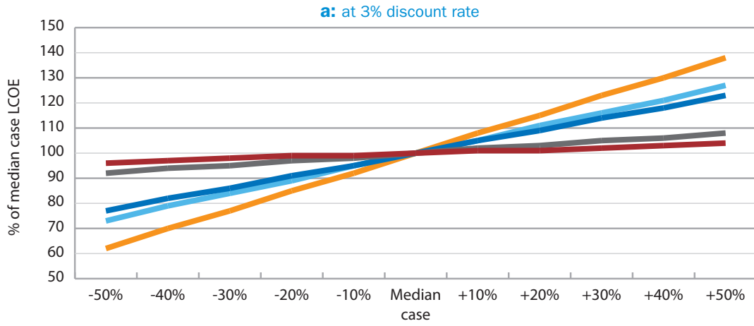
Figure 7.8: LCOE as a function of overnight cost
