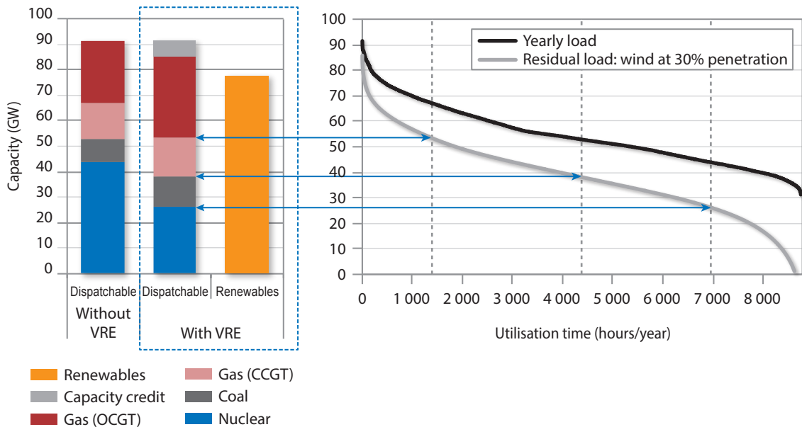
Figure 10.5: Optimal long-term generation mix with and without VRE
