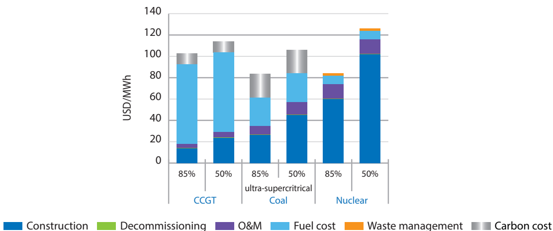
Figure 4.23: LCOE at 85% and 50% capacity factor – Belgium (7% discount rate)
