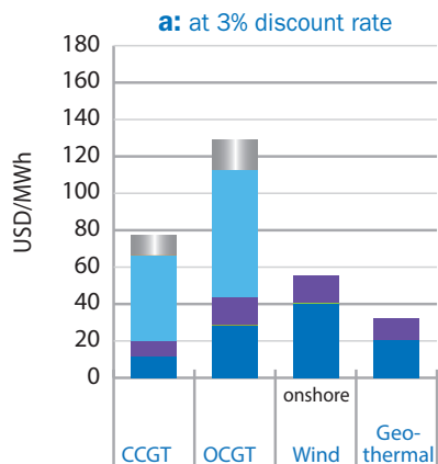
Figure 4.12: Levelised cost of electricity – New Zealand
