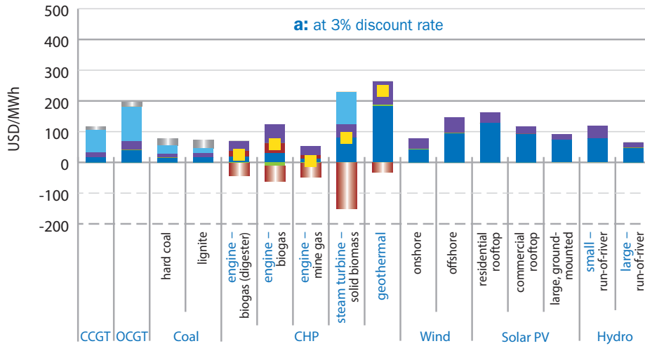
Figure 4.6: Levelised cost of electricity – Germany
