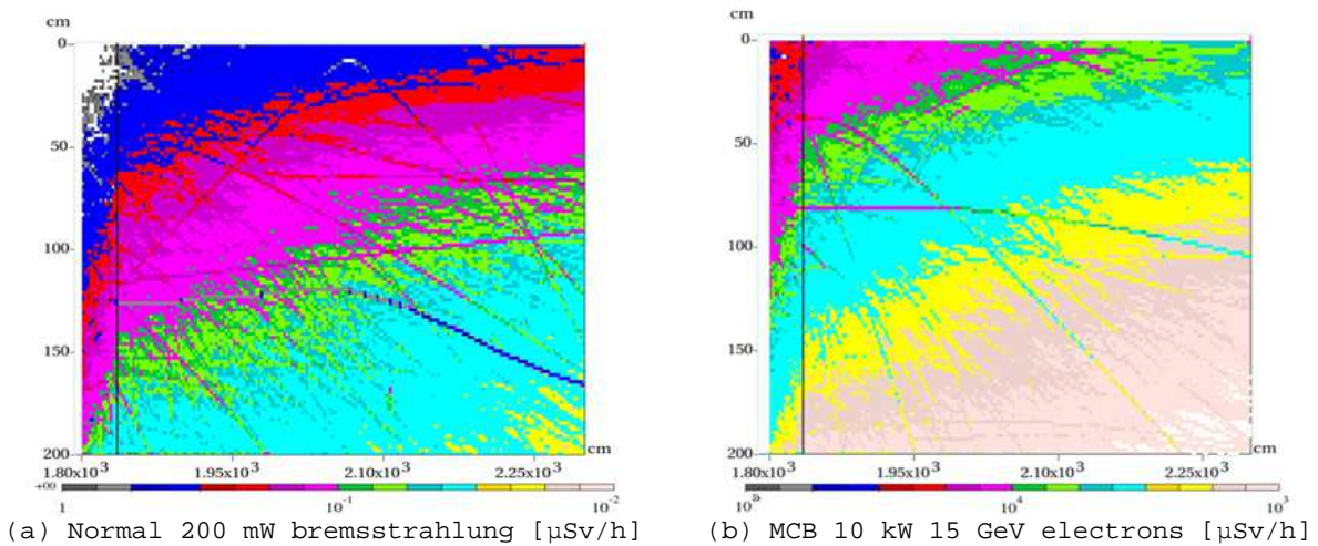
Figure 3: Total dose distribution of SXR with 30 cm thick safety collimator from MARS15 simulations
