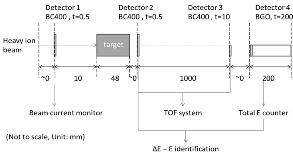
Figure 1: Schematic diagram of the detector system configuration
