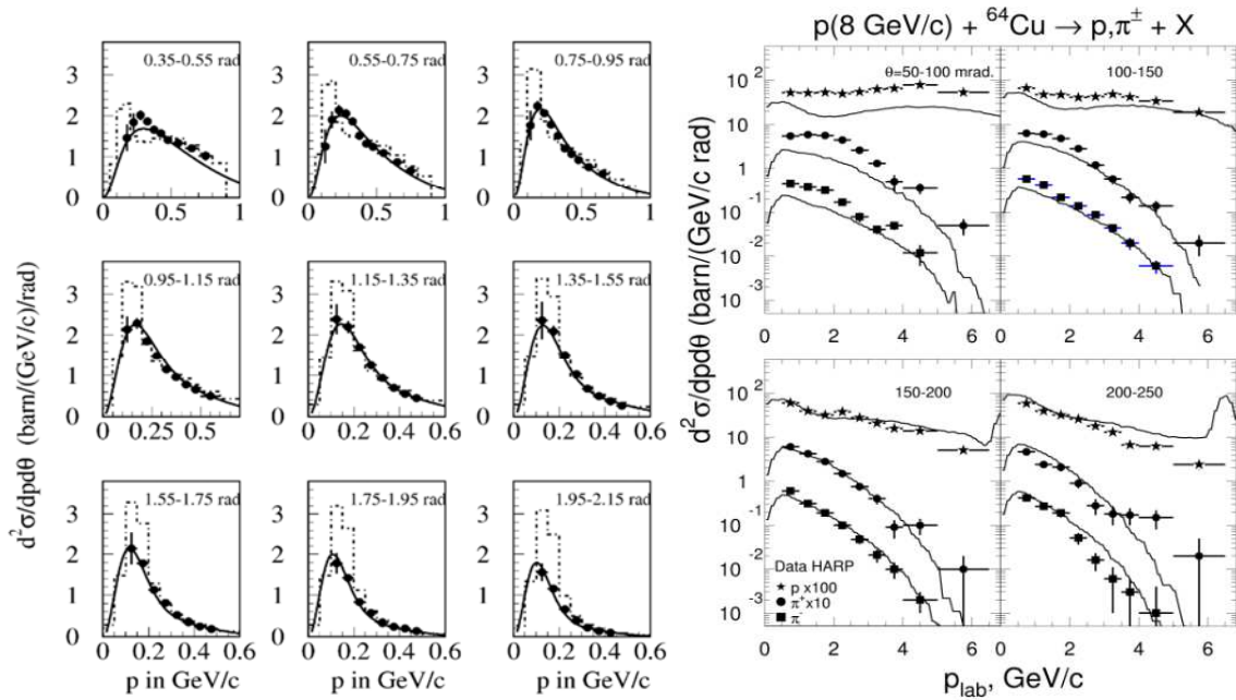
Figure 5: Left: \pi^- production in p+Pb interactions at 8 GeV/c calculated with inclusive (solid) and LAQSM (dashed) models vs HARP data [9]
