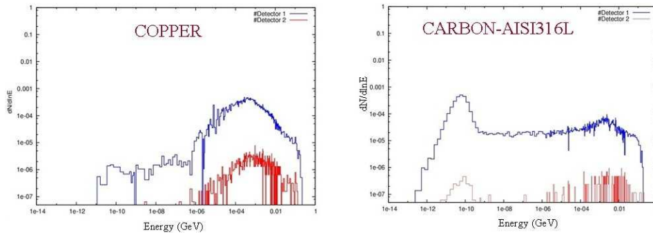
Figure 13: Spectra of the neutrons (neutrons \text{sr}^{-1} per primary proton) coming out from the dump in the backward direction, for the two studied models of the beam dump
