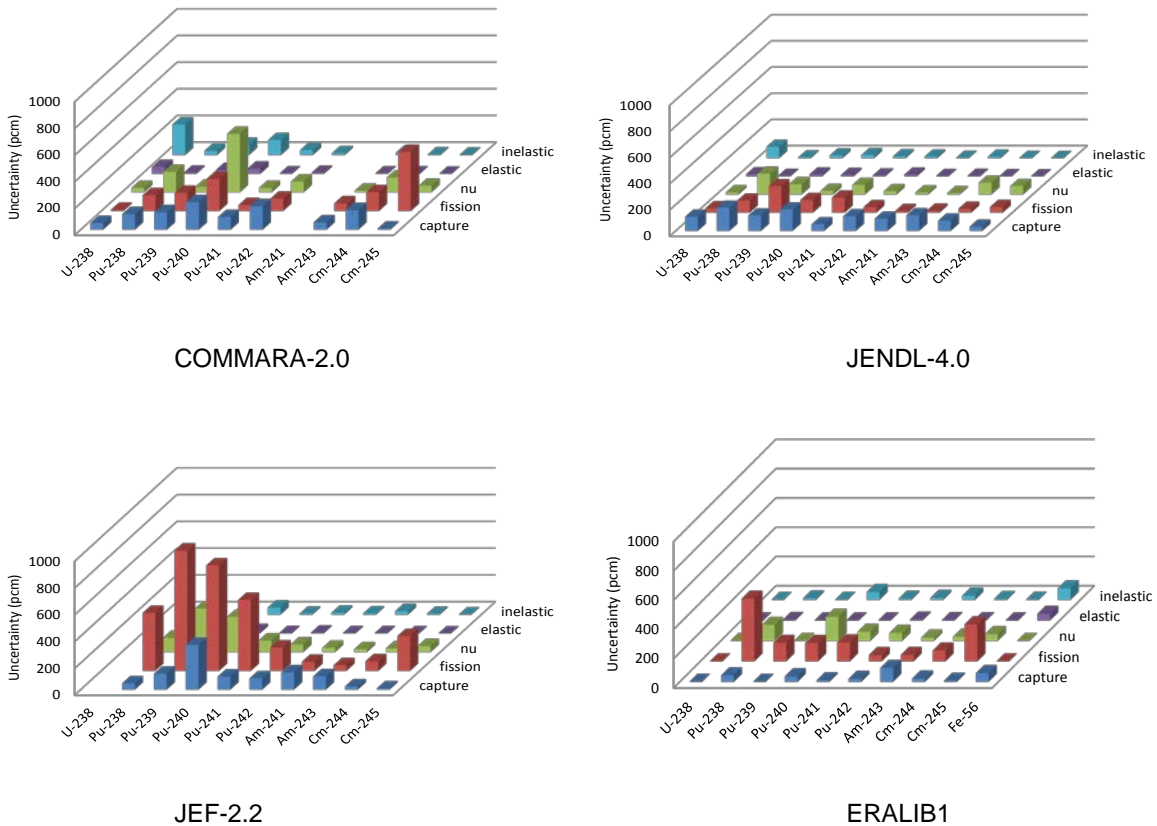
Figure 9: Uncertainty analysis results for k_{\text{eff}} of SFR (actinide isotopes)
