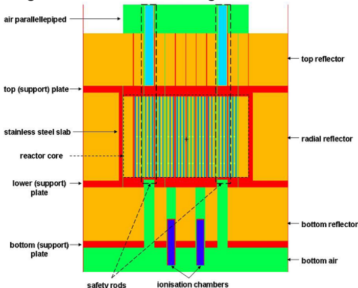
Figure 46: Axial section through the VENUS-F reactor
