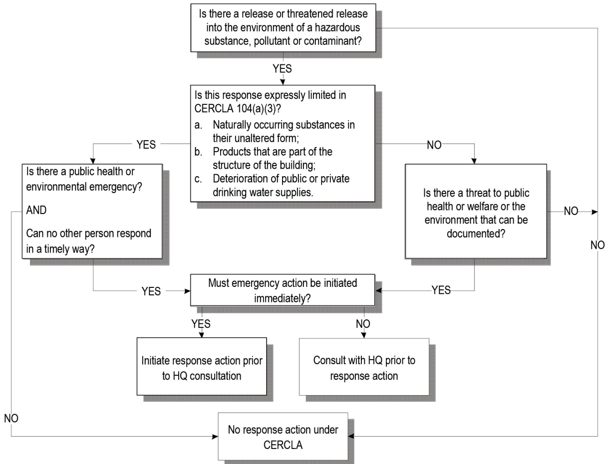
Figure D1. Indoor contamination: Steps for action
