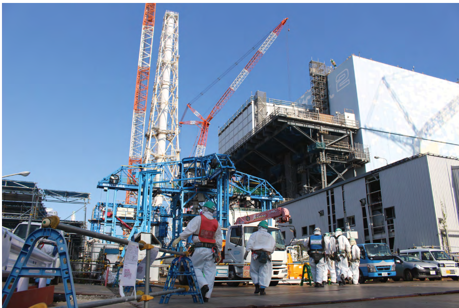
Workers heading to south of the Unit 2 reactor building of the Fukushima Daiichi Nuclear Power Plant to install the adjoining platform. Source: TEPCO Holdings
