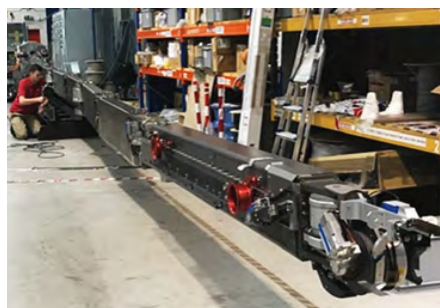
Robot arm part of the system to be used for the trial retrieval of fuel debris inside the Unit 2 primary containment vessel at the Fukushima Daiichi Nuclear Power Plant. It was developed in the United Kingdom and after being shipped to Japan, it will be used once its performance is confirmed and operators are trained with the help of a simulator. Source: International Research Institute for Nuclear Decommissioning (IRID)
