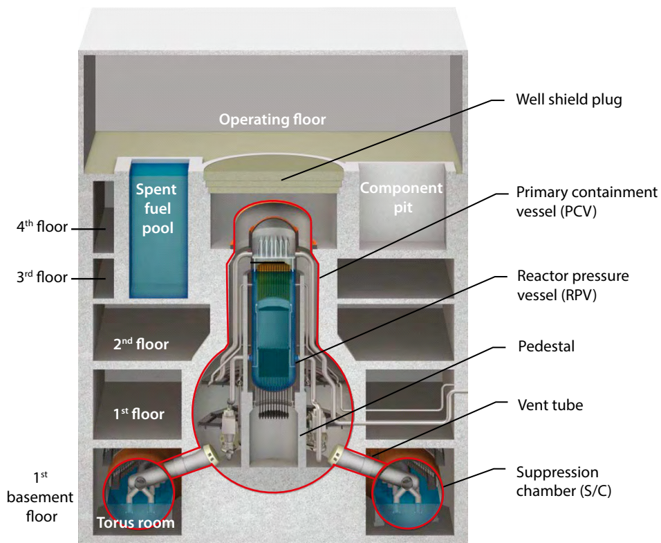
Figure 1.1: Basic design of Fukushima Daiichi boiling water reactors
