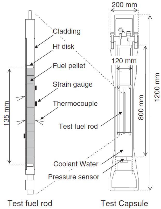
Figure 6. Test fuel rod and test capsules
